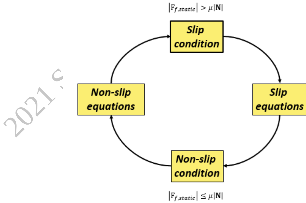
Figure 12: Stick-slip transition model.
