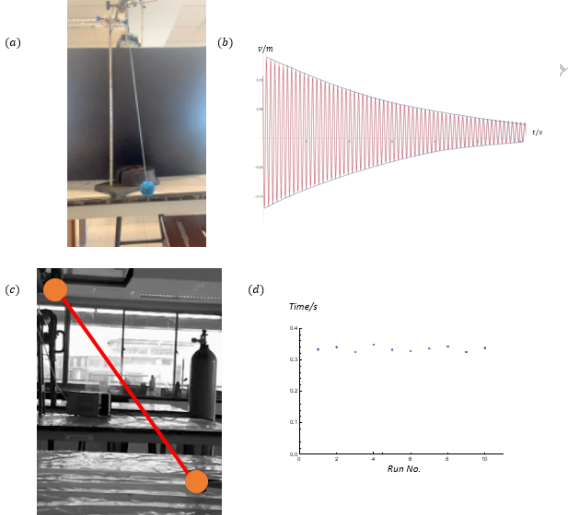
Figure 3: Experimental setup for constant characterization. (a) Experimental setup to measure drag coefficient. A single ball is set up as a simple pendulum and set into oscillation with small displacement. (b) Displacement-time graph of the pendulum. Fitting the decay envelope to the displacement-time graph of the pendulum, we could obtain the drag coefficient. (c) Setup to measure static and kinetic friction coefficients. Adjust the tilted angle of the string and measure the angle which the ball just starts to slide downwards to obtain the static friction coefficient. Track the displacement of the movement of the ball and measure its velocity for calculation of friction force based on force equilibrium. (d) Velocity of ball across multiple experiments.
