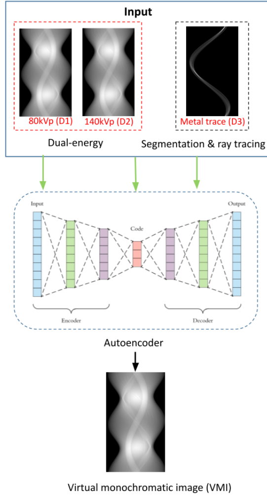
Figure 8: The triple-entry, single-out architecture of the MAR network. 3 copies of the input (corrupted dual-energy data and metal mask sinogram) are separately fed into the 3 material decomposition pathways in the convolutional autoencoder to output a VMI image.
