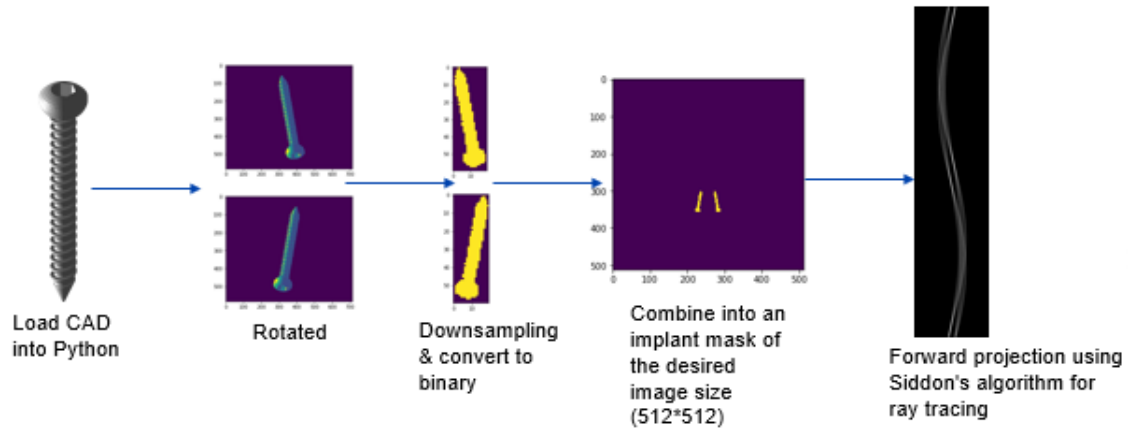
Figure 5: The process of generating a metal implant sinogram from a CAD image.
