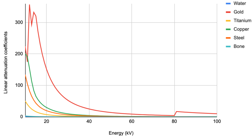
Figure 1: Attenuation coefficient of different materials as a function of energy [46]. The attenuation coefficient of a material is generally correlated with its density.
