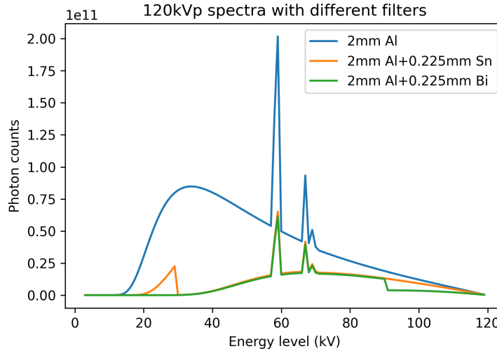
Figure 2: The X-ray spectrum at the 120kV tube voltage when different filters are used. Filters (metal sheets placed between the X-ray beam and the patient) are commonly used to filter out some low-energy photons to partially reduce metal artifacts.
