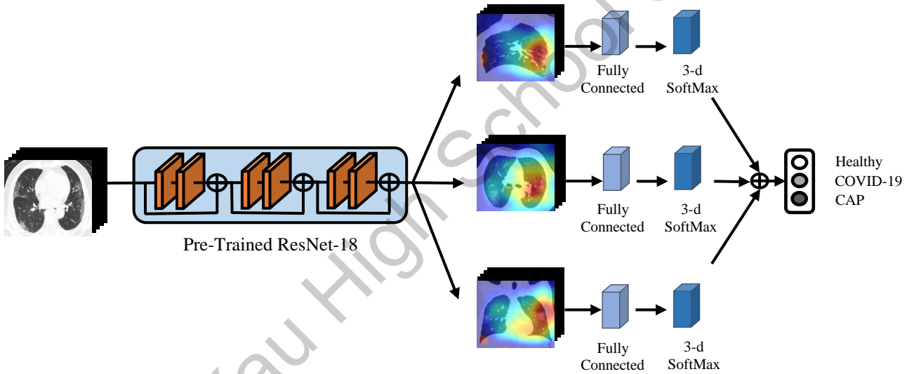
Fig. 5. The details of our proposed Multi-View-Oriented Classifier.
