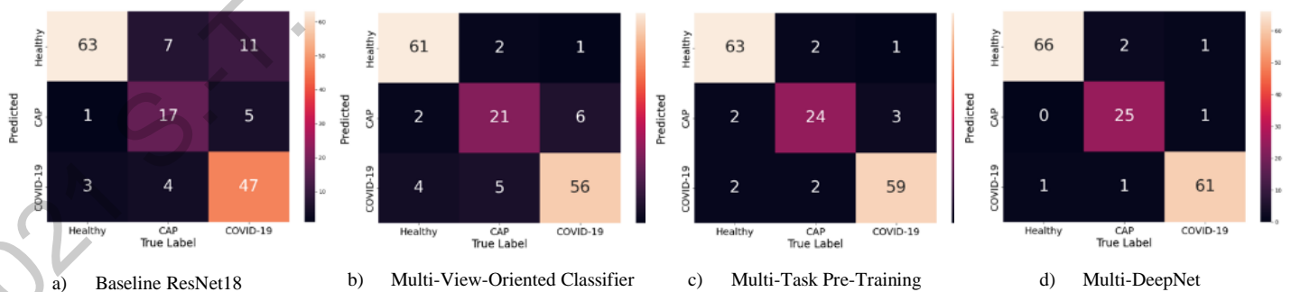
Fig. 6. Confusion matrices are generated to analyze the specific performance of different models on each of the three classes (from left to right: baseline ResNet18, ResNet18 with Multi-View-Oriented Classifier, ResNet18 with Multi-Task Pre-Training, and our proposed Multi-DeepNet).
