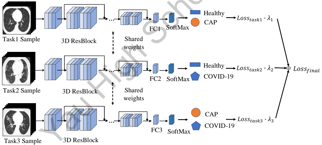
Fig. 4. The details of our multi-task pre-training module.
