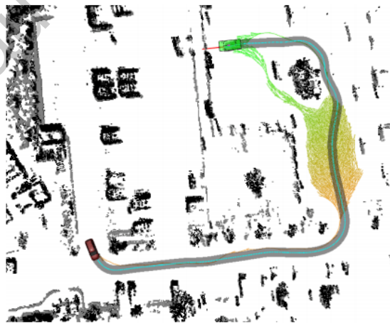
Figure 3: A* algorithm adopted by Leedy and others, in which a local path is built for the autonomous car "Rockey" for the 2005 DARPA Urban Challenge. [13]
