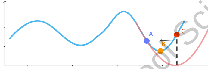
Figure 5: Using the Newton iteration method may lead to overshoot. The position obtained by the current iteration is point A . The red function is our second-order approximation to the blue function, and the Newton iteration goes next to the position of the lowest value under the current approximation, which is the position of point C . But this position is off from the true lowest point B .
