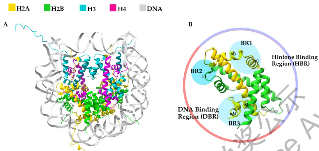
Figure 1 The structure of nucleosome and H2A-H2B dimer.
