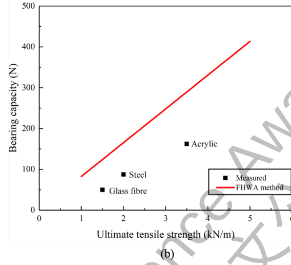
Fig. 7. Comparison between FHWA-predicted and measured bearing capacity: (a) effect of geogrid spacing; (b) effect of geogrid tensile strength.
