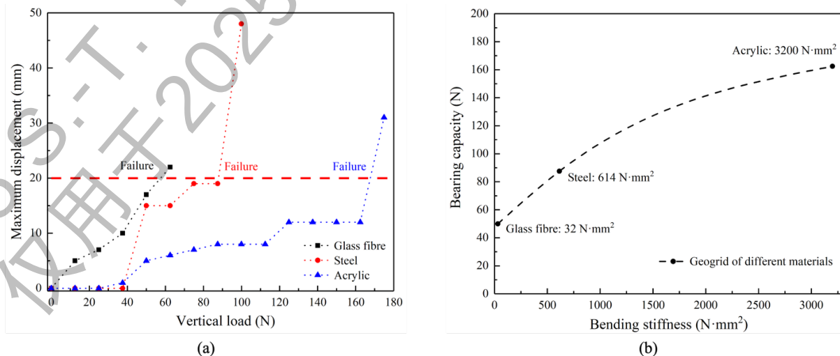
Fig. 6. Effect of geogrid material on bearing capacity: (a) maximum displacement point of facing wall (dashed line represents failure threshold); (b) bearing capacity under different reinforcement material bending stiffness.
