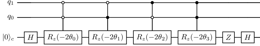
Figure 1: The imaginary diagonal block encoding for N = 4 .
