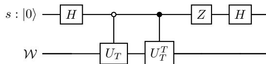
Figure 4: The block-encoding circuit for \mathfrak{so}_{2n}(\mathbb{C}) and \mathfrak{so}_{2n+1}(\mathbb{C}) .
