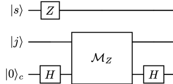
Figure 8: Block-encoding circuit for a type- C_n Cartan element.
