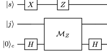
Figure 9: Block-encoding circuit for a type- D_n Cartan element.
