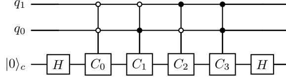
Figure 2: The block encoding of a complex diagonal matrix for N = 4 .
