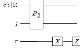
Figure 7: Block-encoding circuit for a type- B_n Cartan element.
