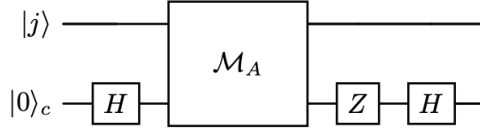
Figure 6: Block-encoding circuit for a type- A_{n-1} Cartan element.
