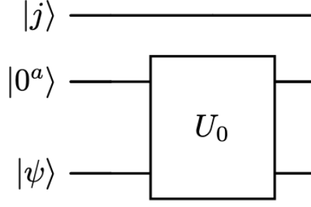
Figure 11: The repeated-block encoding.
