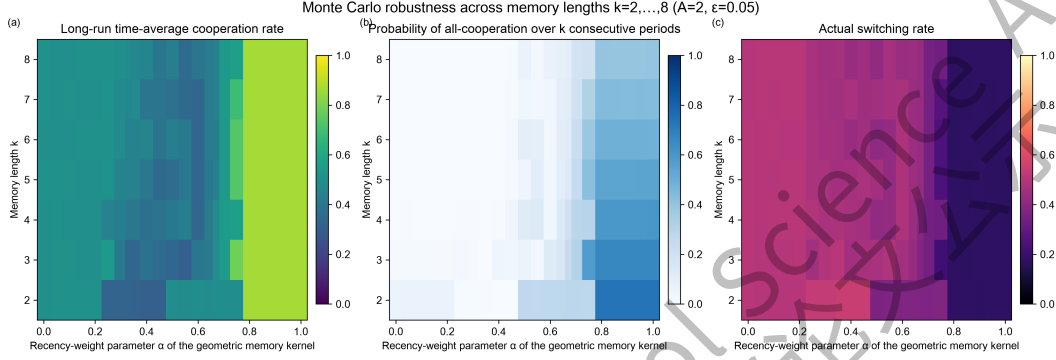
Fig. 9: Robustness of the high-recent-weight mechanism across different memory lengths. The three panels correspond to (a) long-run cooperation rate, (b) probability of mutual cooperation over k consecutive rounds, and (c) actual switching rate.
