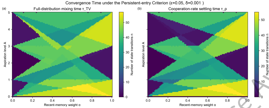
Fig. 19: Convergence time under criterion \delta = 0.001 over \alpha and A
