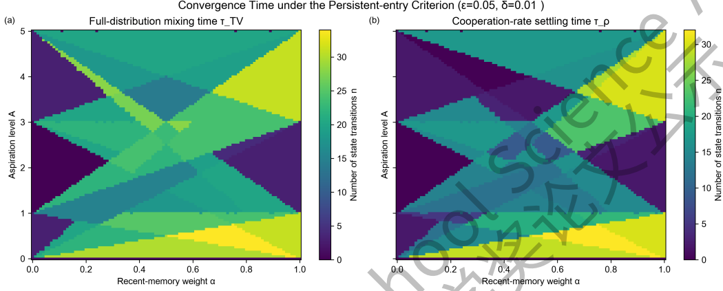
Fig. 18: Convergence time under criterion \delta = 0.01 over \alpha and A
