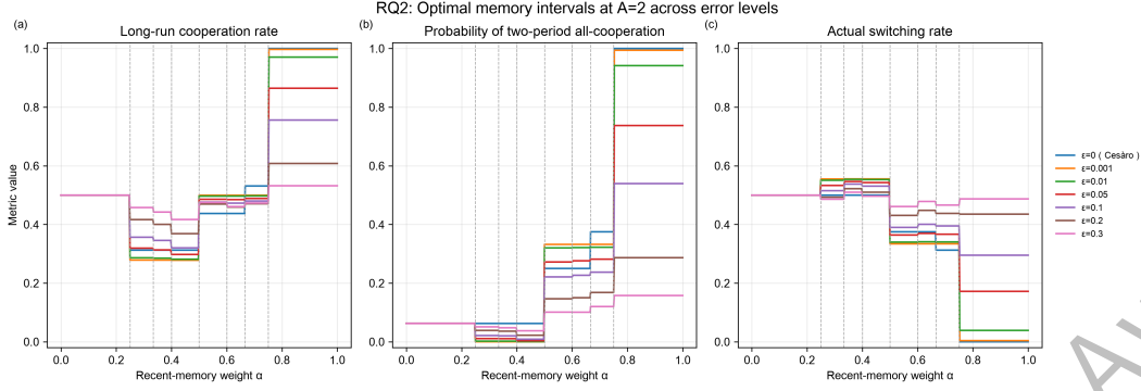
Fig. 20: Long-run cooperation rate \rho_\infty (panel a), stationary probability of CCCC (panel b), and actual switching rate \sigma_{\text{actual}} (panel c) as functions of \alpha and \varepsilon at A = 2 . The vertical dashed lines mark the theoretical critical values of \alpha .
