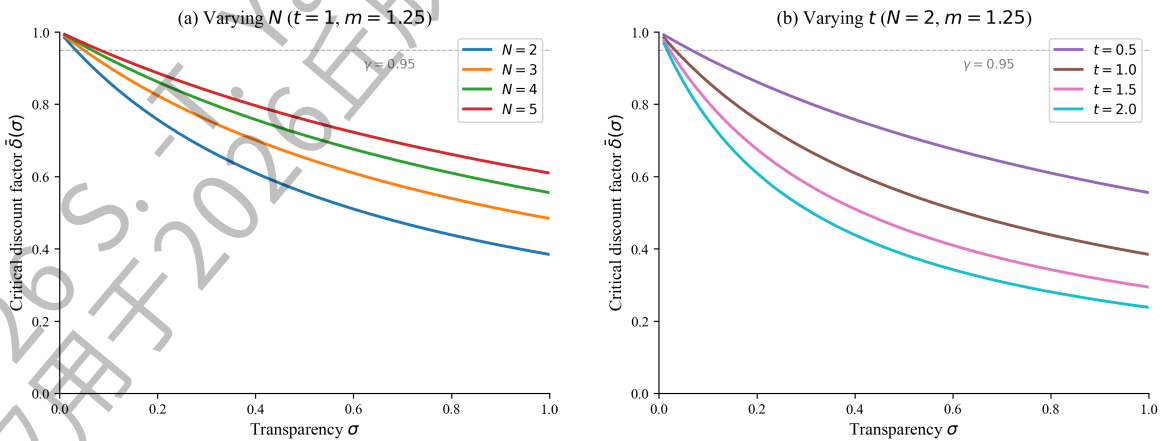
Figure 4: Critical discount factor \bar{\delta}(\sigma) under varying N and t .
