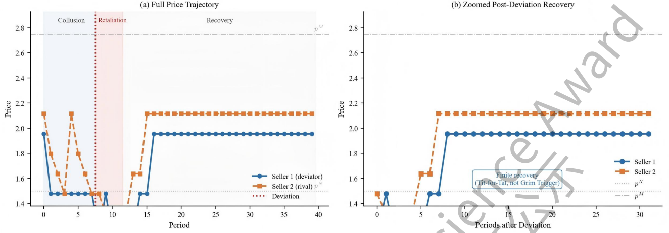
Figure 5: Punishment-recovery dynamics after forced unilateral price deviation ( N = 2 , \gamma = 0.95 , \sigma = 1.0 ).
