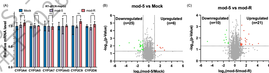
Figure 8 Evaluation of the off-target effects of chemically modified siRNA. (A) Relative mRNA expression level of CYP3A4, CYP3A5, CYP3A7, CYP3A43, CYP2C9, CYP2D6 in HepG2 cells after transfection with 10nM mod-5 and mod-R. (B) Proteomic analysis of HepG2 cells 48h after transfecting with 10nM mod-5 or Mock. (C) Proteomic analysis of HepG2 cells 48h after transfecting with 10nM mod-5 or mod-R.
