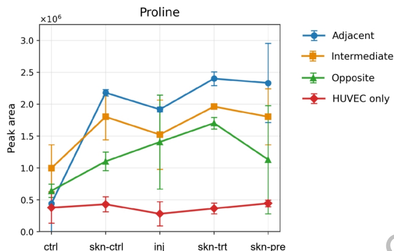
Figure 5 Line graph of proline metabolism in different treatment groups.
