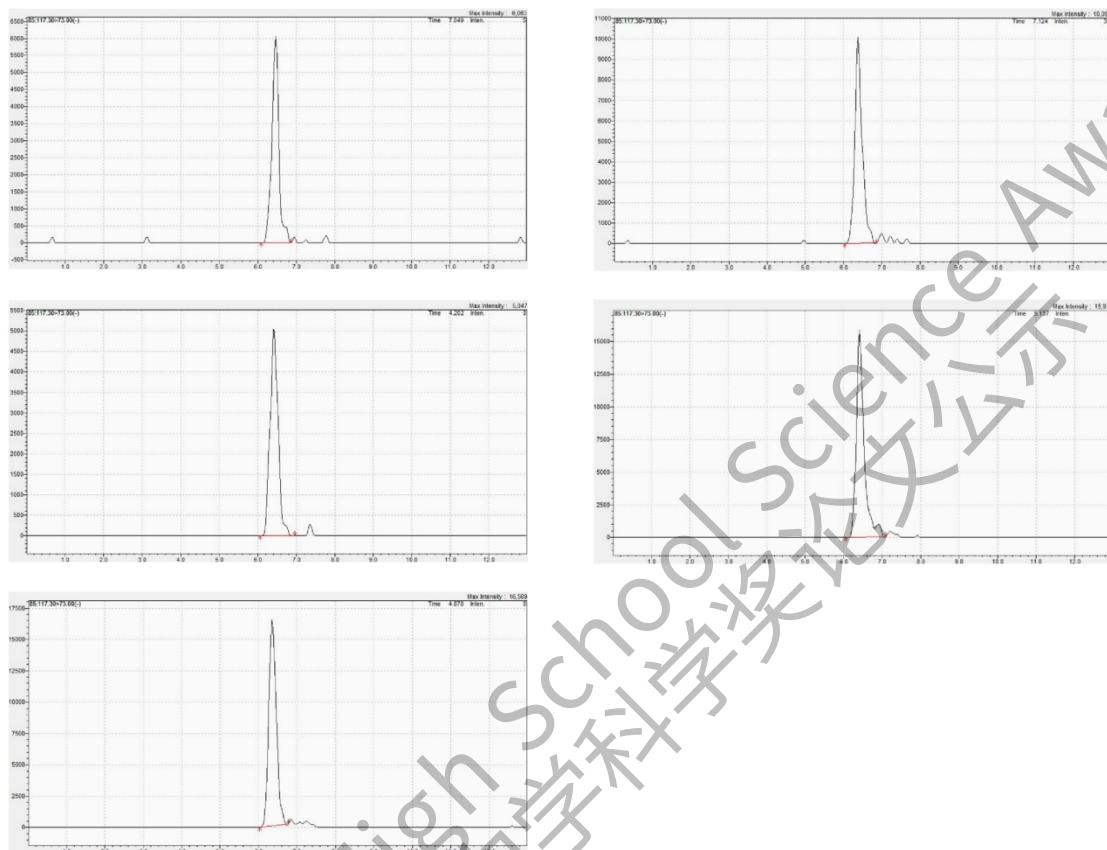
Figure S1 Example of LC-MS extracted ion chromatogram analysis method. The x-axis is retention time, and the y-axis is ion abundance. Substances with identifiable, baseline-separated chromatographic peaks in the extracted ion chromatogram were analyzed. During analysis, the target peak was integrated to obtain the peak area. The peak area can qualitatively reflect the content of the corresponding substance.
